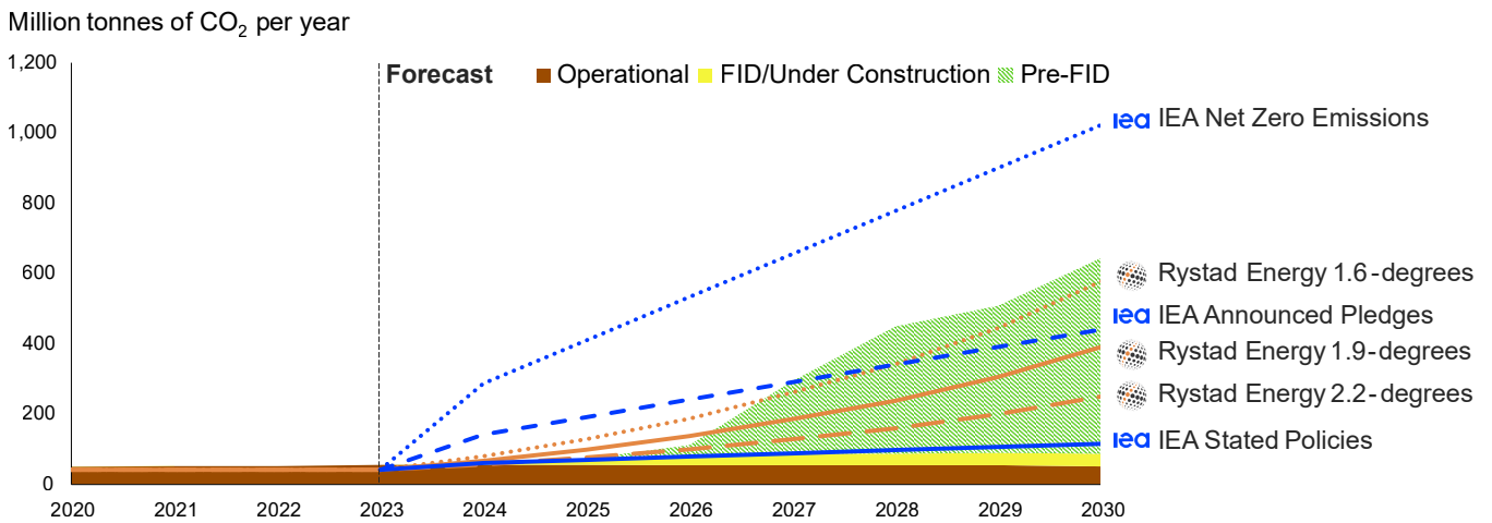
Figure 6: Global unrisked CO 2 capture capacity, known vs aspired
