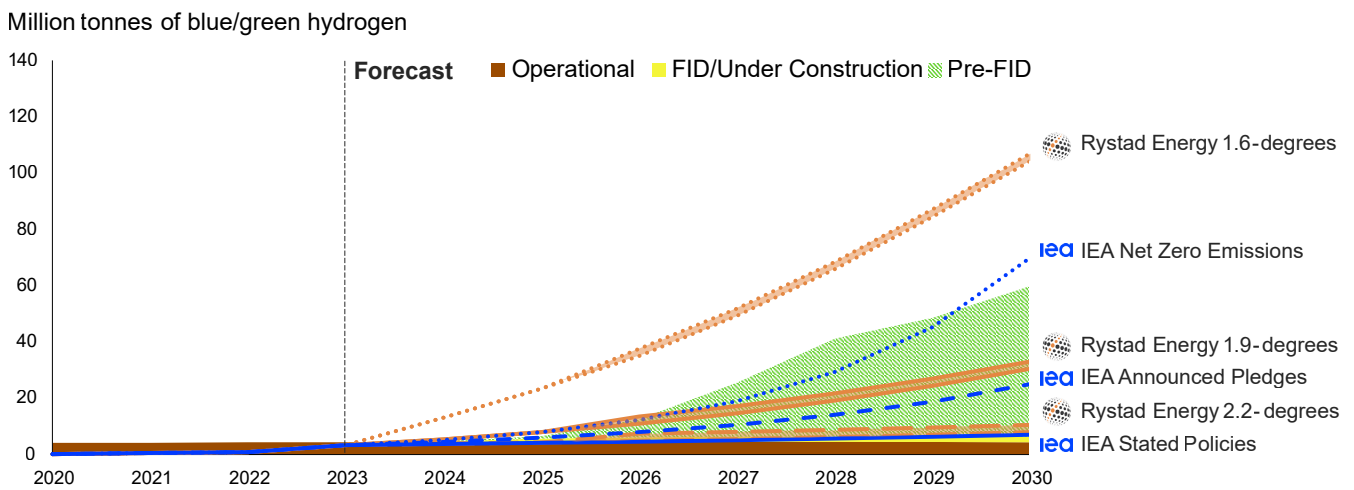
Figure 5: Global unrisks zero- and low-CO 2 hydrogen production capacity, known vs. aspired
